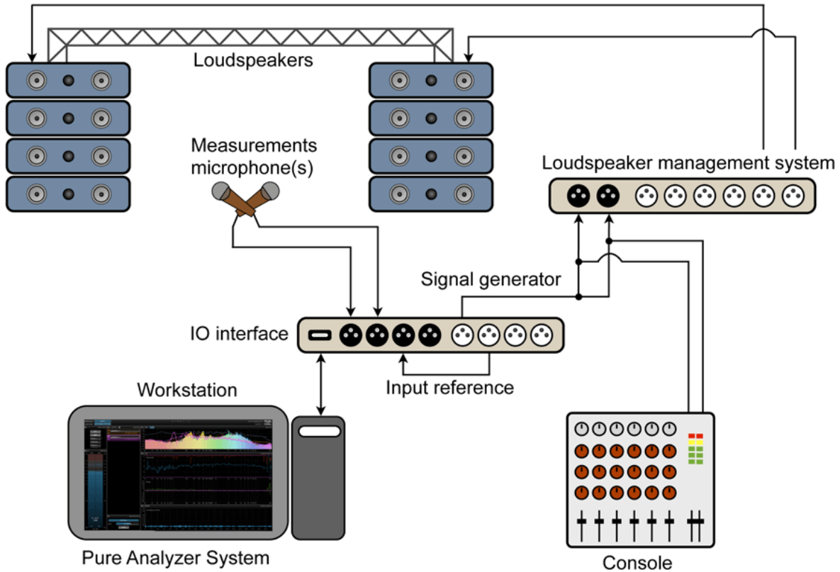
Figure 27.2: Typical configuration for a live venue measurement setup using FLUX:: Analyzer’s internal signal generator and loopback
