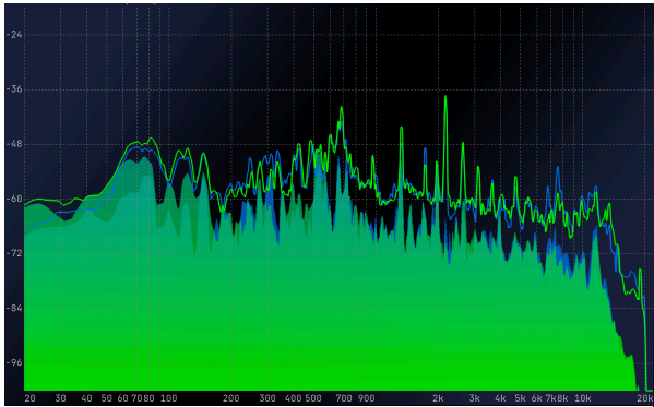
(a) Magnitude spectrum of a stereo signal with summing disabled, max and smoothed curves enabled
