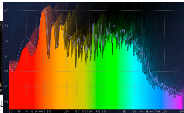
(a) Magnitude spectrum with "Slide" option enabled (Real time waterfall)
